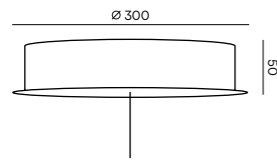
Canopy for PC1291 incl. PWM dimming system
