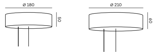
Canopy for PWM dimming system
