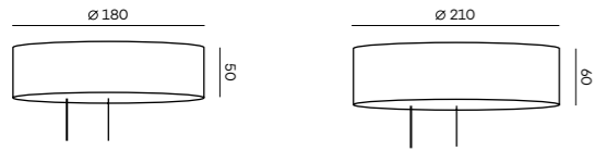
Canopy for PWM dimming system
